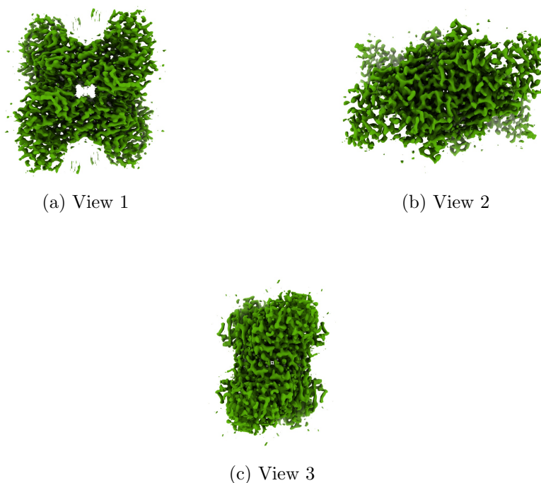
Figure 4: Isosurface at threshold=0.828000. Views generated by ChimeraX at the following X, Y, Z angles: View 1 (0, -90, -90), View 2 (-90, 0, -90), View 3 (0, 0, 0).
