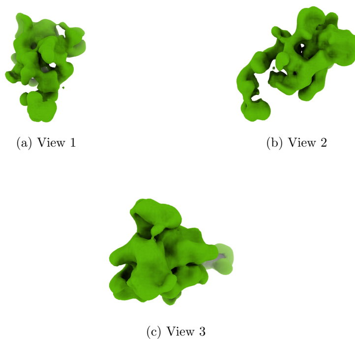
Figure 4: Isosurface at threshold=0.075000. Views generated by ChimeraX at a the following X, Y, Z angles: View 1 (0, -90, -90), View 2 (-90, 0, -90), View 3 (0, 0, 0).
