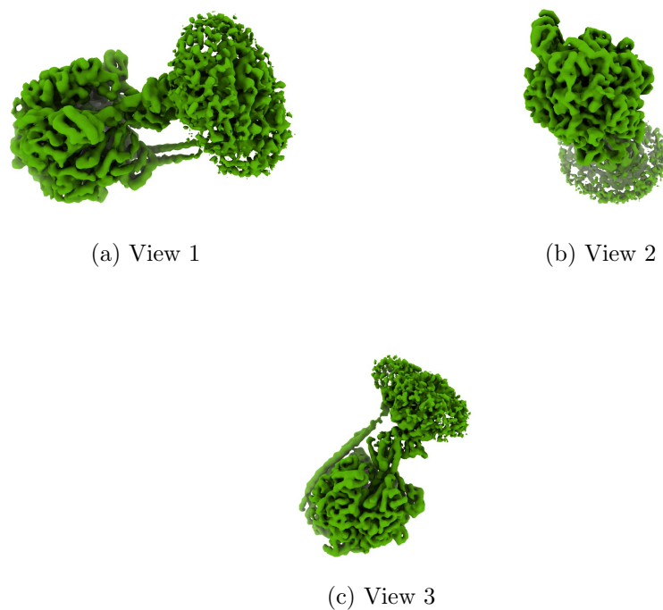
Figure 4: Isosurface at threshold=0.451000. Views generated by ChimeraX at a the following X, Y, Z angles: View 1 (0, -90, -90), View 2 (-90, 0, -90), View 3 (0, 0, 0).
