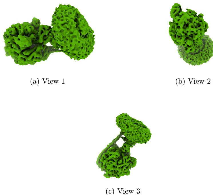
Figure 4: Isosurface at threshold=0.327000. Views generated by ChimeraX at a the following X, Y, Z angles: View 1 (0, -90, -90), View 2 (-90, 0, -90), View 3 (0, 0, 0).
