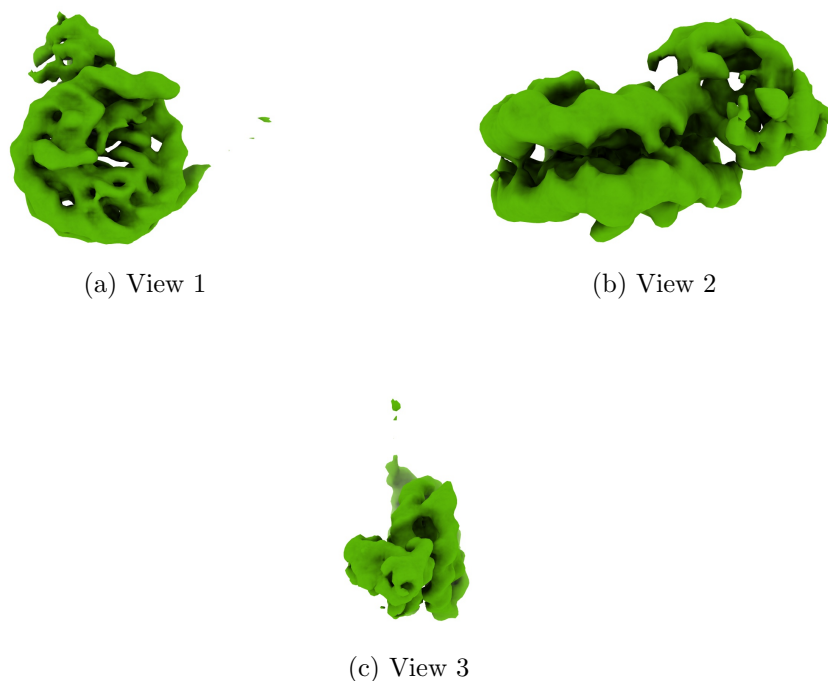
Figure 4: Isosurface at threshold=1.300000. Views generated by ChimeraX at a the following X, Y, Z angles: View 1 (0, -90, -90), View 2 (-90, 0, -90), View 3 (0, 0, 0).
