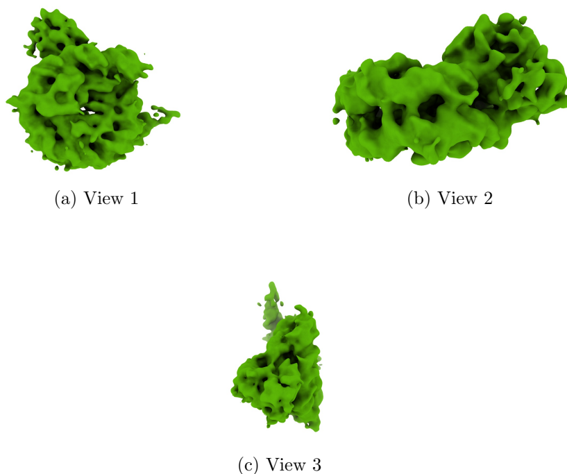
Figure 4: Isosurface at threshold=0.200000. Views generated by ChimeraX at a the following X, Y, Z angles: View 1 (0, -90, -90), View 2 (-90, 0, -90), View 3 (0, 0, 0).
