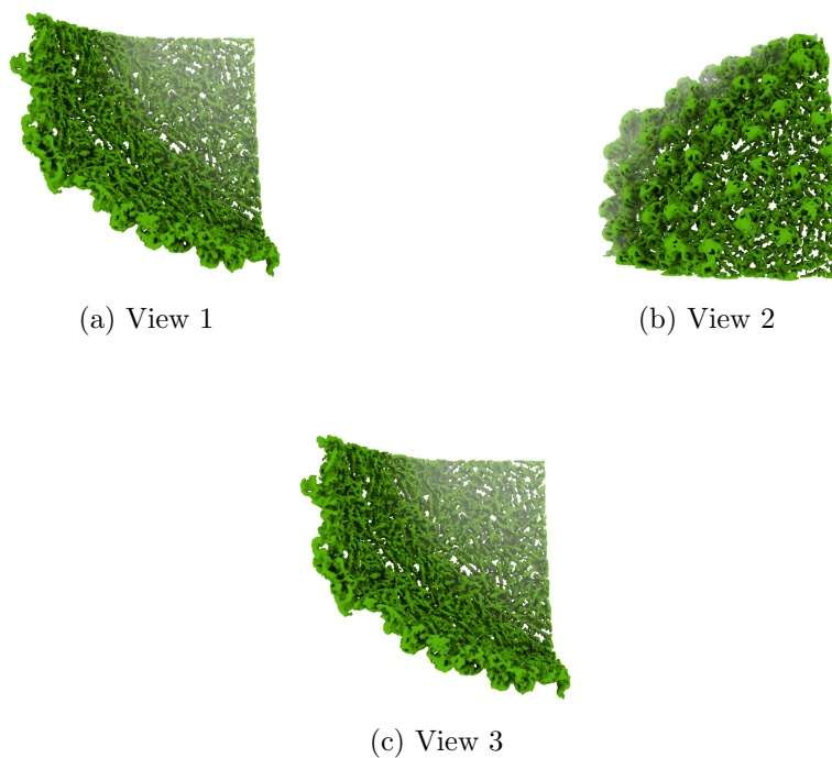
Figure 4: Isosurface at threshold=2.180000. Views generated by ChimeraX at a the following X, Y, Z angles: View 1 (0, -90, -90), View 2 (-90, 0, -90), View 3 (0, 0, 0).
