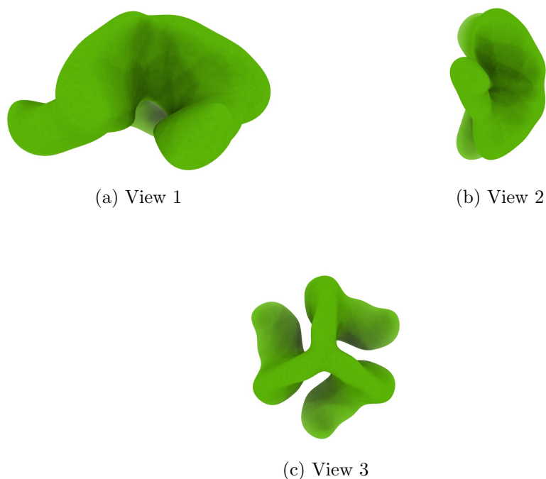
Figure 4: Isosurface at threshold=2.130000. Views generated by ChimeraX at a the following X, Y, Z angles: View 1 (0, -90, -90), View 2 (-90, 0, -90), View 3 (0, 0, 0).
