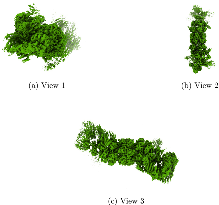
Figure 4: Isosurface at threshold=0.034000. Views generated by ChimeraX at a the following X, Y, Z angles: View 1 (0, -90, -90), View 2 (-90, 0, -90), View 3 (0, 0, 0).
