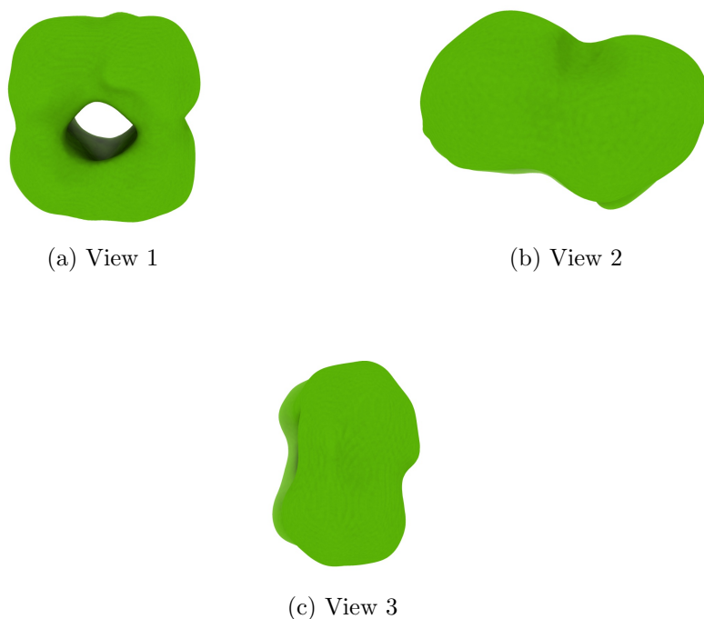
Figure 4: Isosurface at threshold=0.136000. Views generated by ChimeraX at a the following X, Y, Z angles: View 1 (0, -90, -90), View 2 (-90, 0, -90), View 3 (0, 0, 0).
