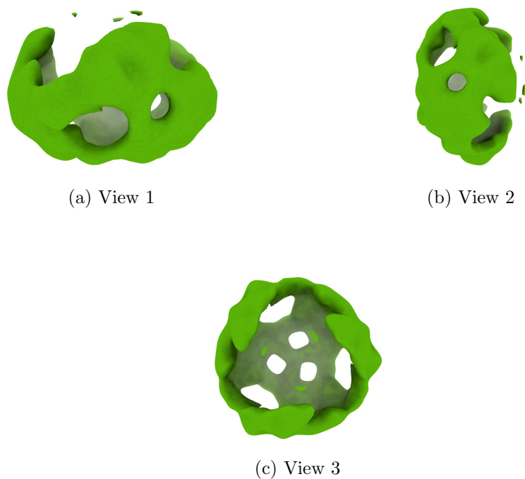
Figure 4: Isosurface at threshold=0.199000. Views generated by ChimeraX at a the following X, Y, Z angles: View 1 (0, -90, -90), View 2 (-90, 0, -90), View 3 (0, 0, 0).
