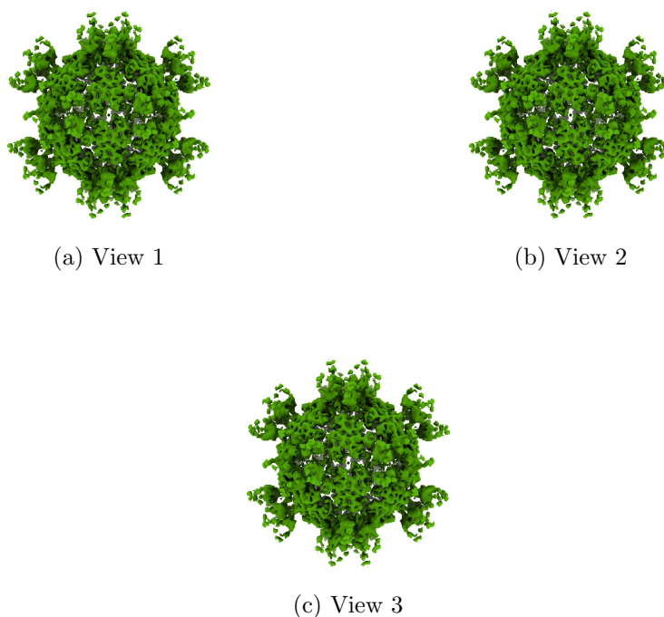
Figure 4: Isosurface at threshold=22.000000. Views generated by ChimeraX at a the following X, Y, Z angles: View 1 (0, -90, -90), View 2 (-90, 0, -90), View 3 (0, 0, 0).
