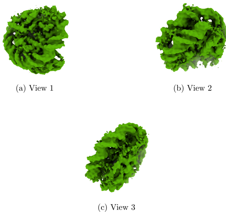
Figure 4: Isosurface at threshold=0.037700. Views generated by ChimeraX at a the following X, Y, Z angles: View 1 (0, -90, -90), View 2 (-90, 0, -90), View 3 (0, 0, 0).
