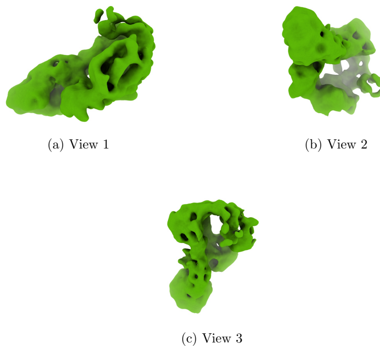
Figure 4: Isosurface at threshold=0.928000. Views generated by ChimeraX at a the following X, Y, Z angles: View 1 (0, -90, -90), View 2 (-90, 0, -90), View 3 (0, 0, 0).
