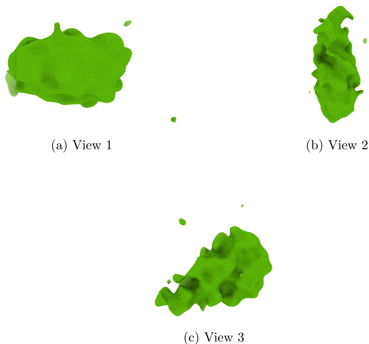
Figure 4: Isosurface at threshold=0.898000. Views generated by ChimeraX at a the following X, Y, Z angles: View 1 (0, -90, -90), View 2 (-90, 0, -90), View 3 (0, 0, 0).
