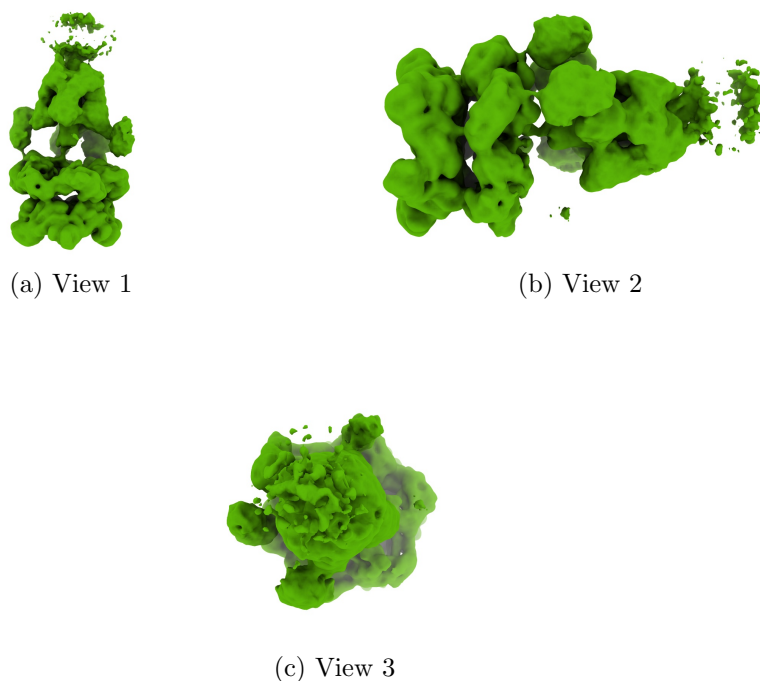
Figure 4: Isosurface at threshold=0.009500. Views generated by ChimeraX at a the following X, Y, Z angles: View 1 (0, -90, -90), View 2 (-90, 0, -90), View 3 (0, 0, 0).
