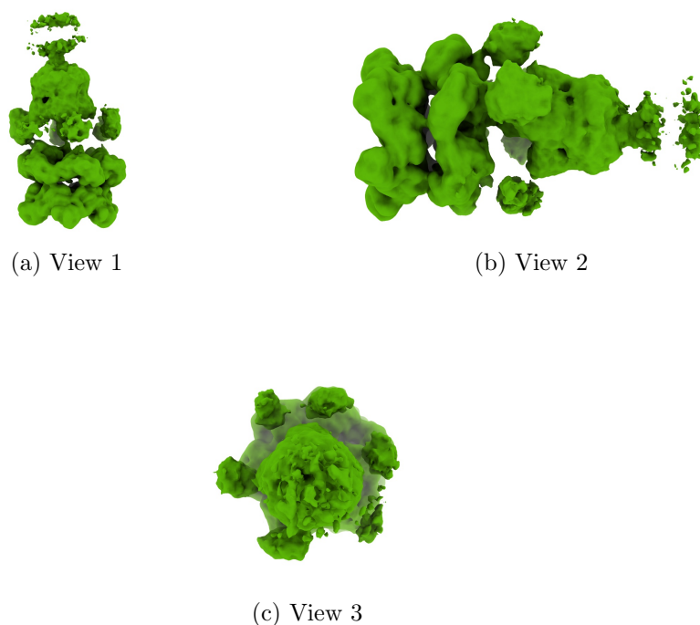
Figure 4: Isosurface at threshold=0.008630. Views generated by ChimeraX at a the following X, Y, Z angles: View 1 (0, -90, -90), View 2 (-90, 0, -90), View 3 (0, 0, 0).
