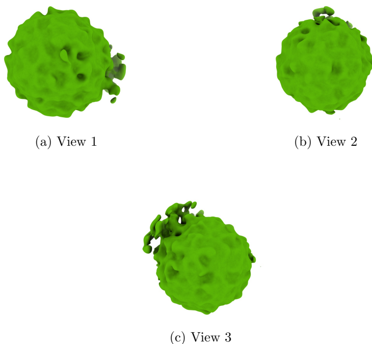
Figure 4: Isosurface at threshold=0.033500. Views generated by ChimeraX at a the following X, Y, Z angles: View 1 (0, -90, -90), View 2 (-90, 0, -90), View 3 (0, 0, 0).
