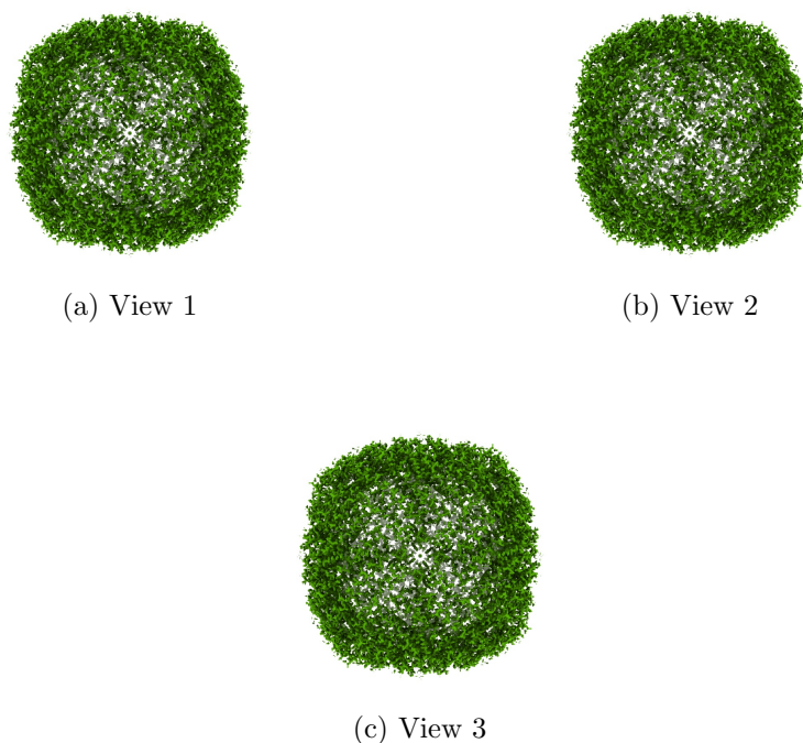
Figure 4: Isosurface at threshold=0.044000. Views generated by ChimeraX at a the following X, Y, Z angles: View 1 (0, -90, -90), View 2 (-90, 0, -90), View 3 (0, 0, 0).
